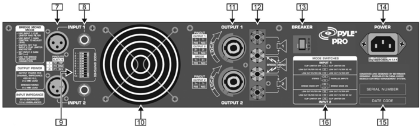
Fig. 2.2: Rear panel control elements
